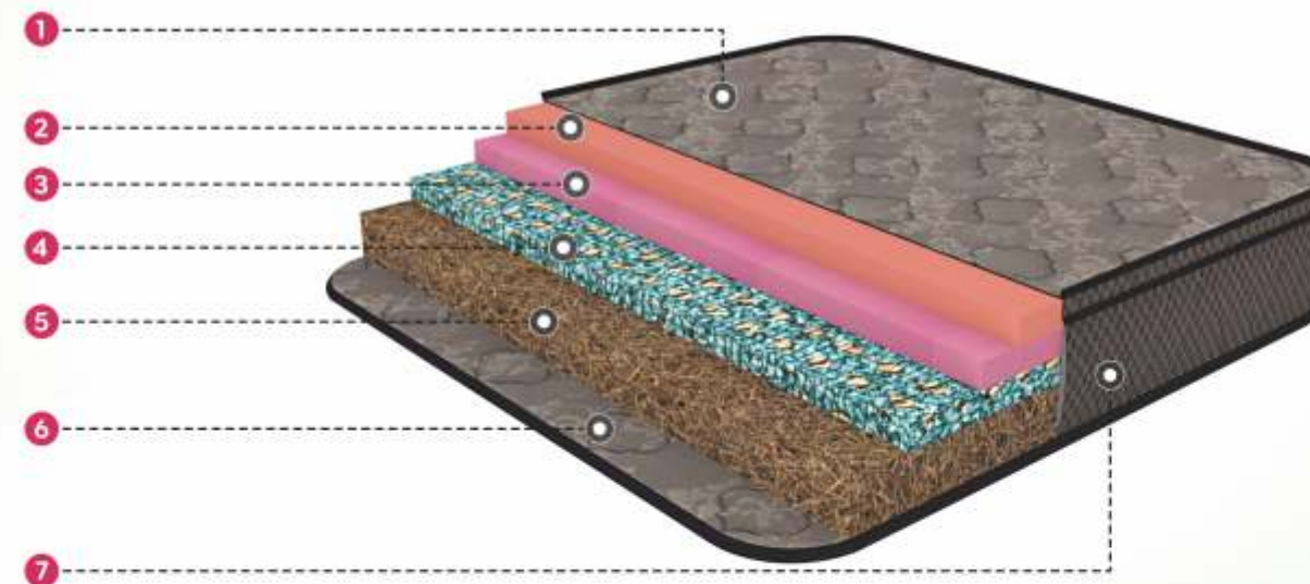
1. Quilt 2. Super Soft Foam 3. PU Foam 4. Bonded Foam 5. Coir 6. Quilt 7. Side Wall Quilt
