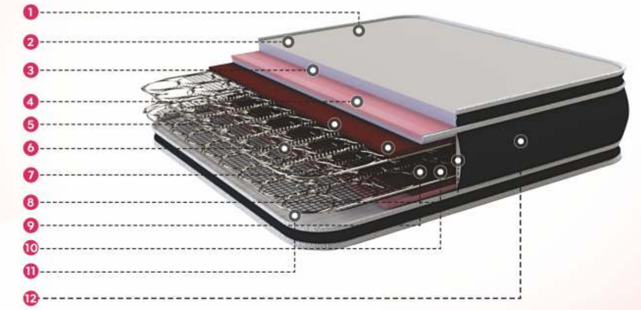
1. Quilt 2. Foam 3. Pillow Top Quilt 4. Cotton Felt 5. Mesh 6. Bonnell Spring 7. Mesh 8. Cotton Felt 9. Pillow Top Quilt 10. Foam 11. Quilt 12. Side Wall Quilt
