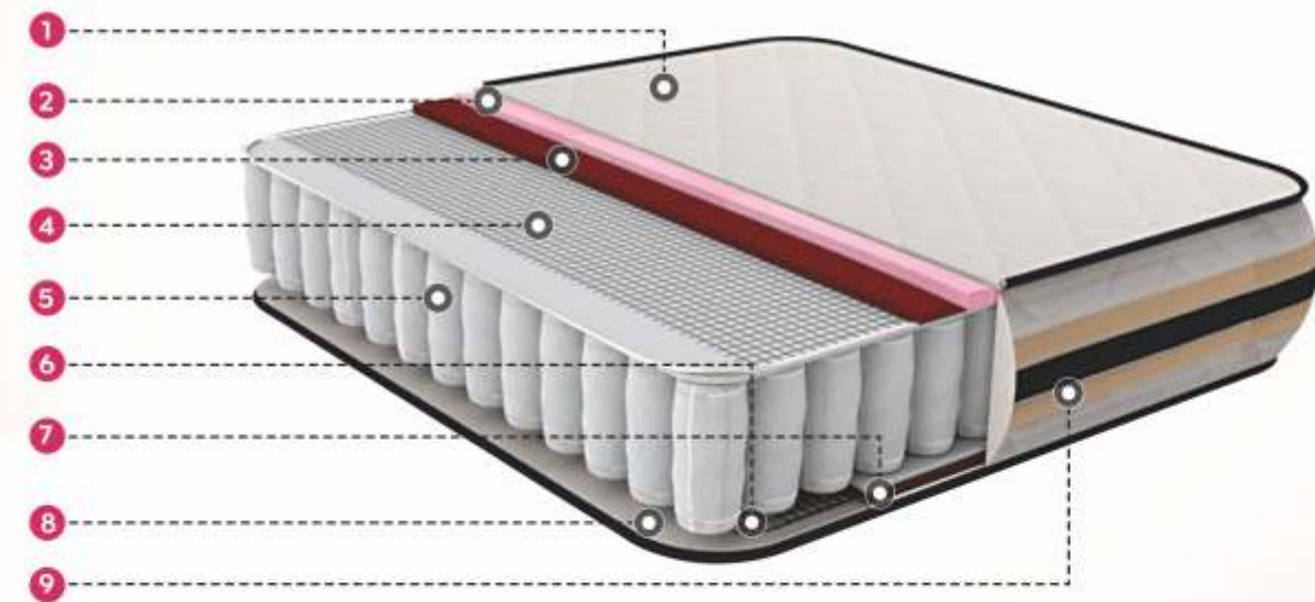
1. Quilt 2. PU Foam 3. Cotton Felt 4. Mesh 5. Pocket Spring 6. Mesh 7. Cotton Felt 8. Quilt 9. Side Wall Quilt
