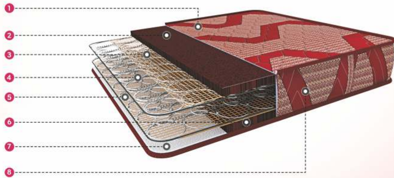
1. Quilt 2. Cotton Felt 3. Mesh 4. Bonnell Spring 5. Mesh 6. Cotton Felt 7. Quilt 8. Side Wall Quilt
