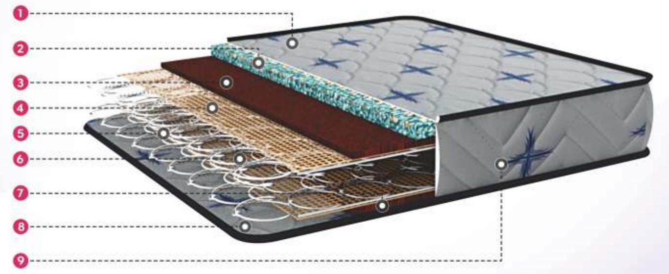
1. Quilt 2. Bonded Foam 3. Cotton Felt 4. Mesh 5. Bonnell Spring 6. Mesh 7. Cotton Felt 8. Quilt 9. Side Wall Quilt
