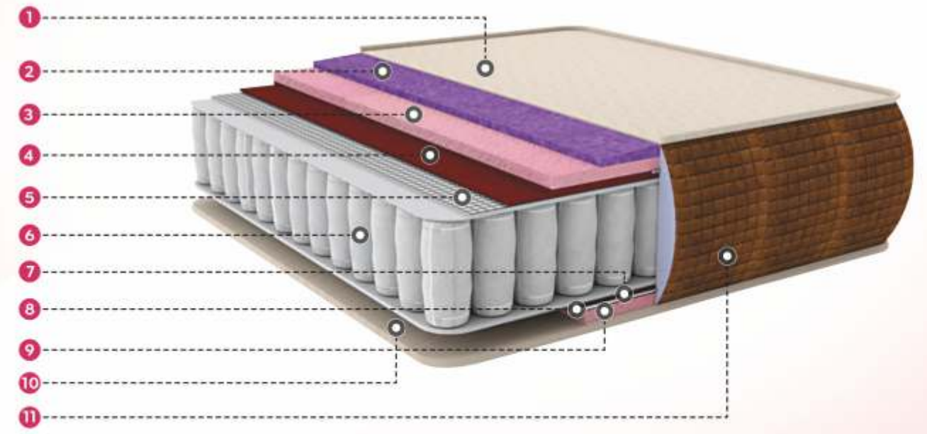
1. Memory Foam Quilt 2. Memory Foam 3. PU Foam 4. Cotton Felt 5. Mesh 6. Pocket Spring 7. Mesh 8. Cotton Felt 9. PU Foam 10. Quilt 11. Side Wall Quilt
