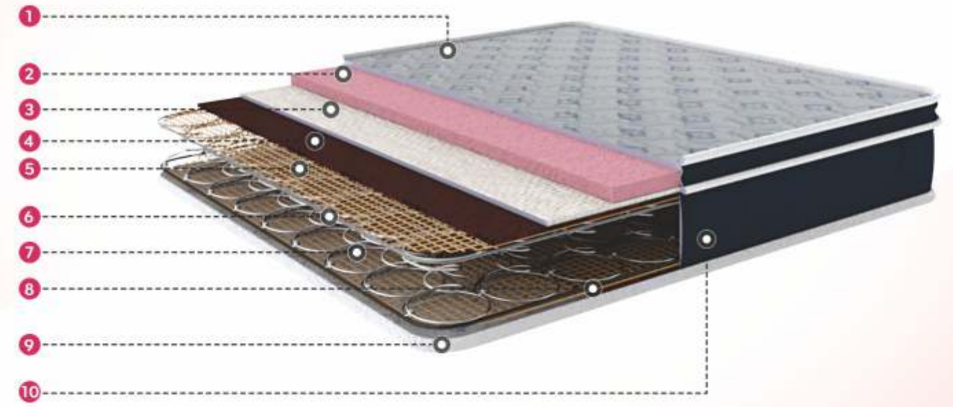
1. Quilt 2. Foam 3. Pillow Top Quilt 4. Cotton Felt 5. Mesh 6. Bonnell Spring 7. Mesh 8. Cotton Felt 9. Quilt 10. Side Wall Quilt
