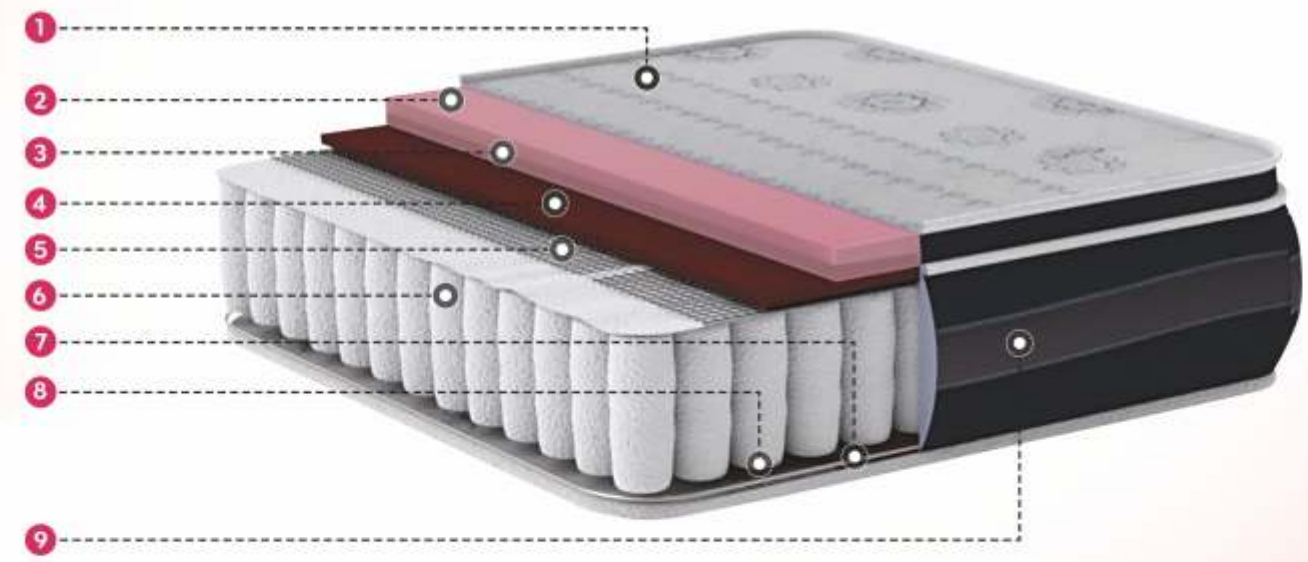
1. Quilt 2. PU Foam 3. Cotton Felt 4. Mesh 5. Pocket Spring 6. Mesh 7. Cotton Felt 8. Quilt 9. Side Wall Quilt
